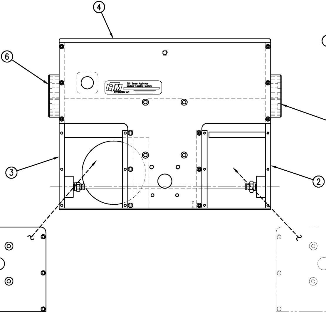
REWIND TRANSITION PLATE~CTM PART #MP-200-0266 ORIENTATION & LOCATION FOR RH APPLICATOR (NOT INCLUDED IN ASSEMBLY)
