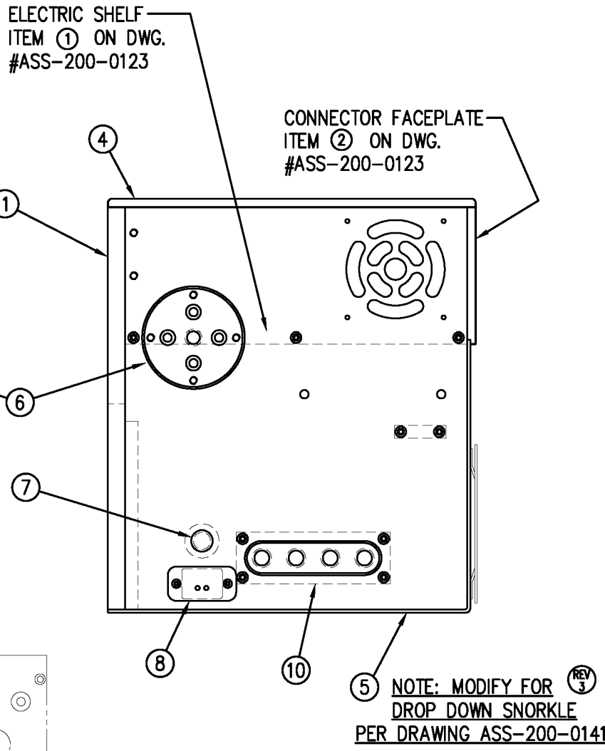
NOTE: ITEMS ⑦ & ⑧ ARE LOCATED ON OPPOSITE SIDE OF HOUSING FOR LH ASSEMBLY.
